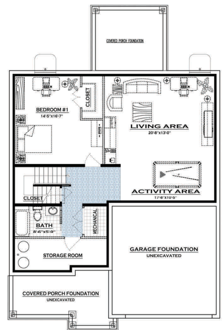
BASEMENT PLAN 1,251 SQ. FT.
