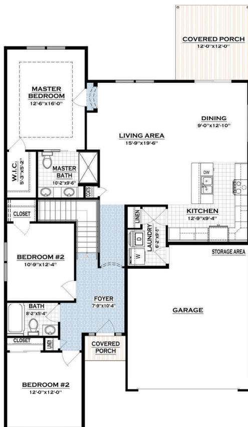
GROUND FLOOR PLAN 1,623 SQ. FT.
